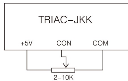
Figure B-3, the application circuit diagram (2) of TRIAC-JKK
