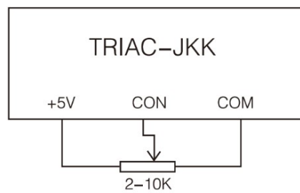
Figure B-2, the application circuit diagram (1) of TRIAC-JKK (Note: see Figure D-B-2 for the improved circuit diagram of Figure B-2)
